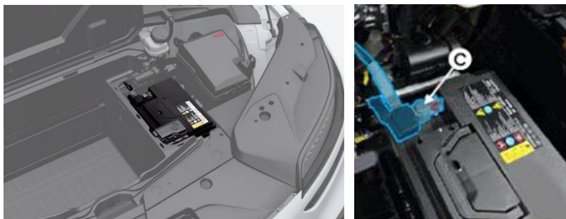
C. Locate the 12 V auxiliary battery and disconnect the (-) cable (C).
