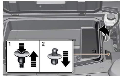
B. Disengage the screw clip and remove the battery service cover.
