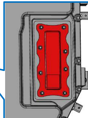
BMS ECU Service Cover
